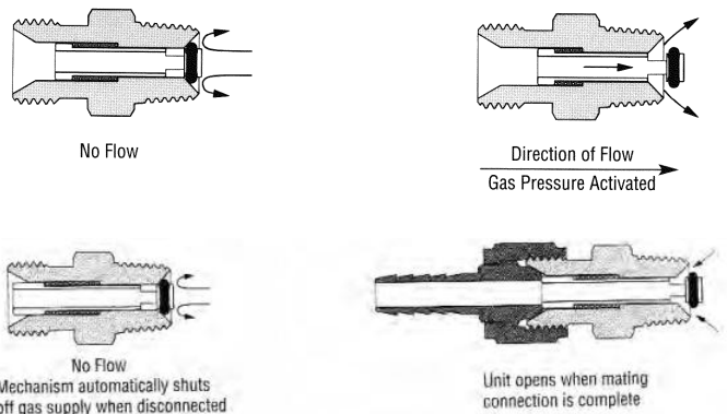
#69-21256 - Typical Operation
